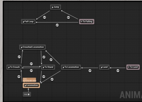
Animation Blueprint
